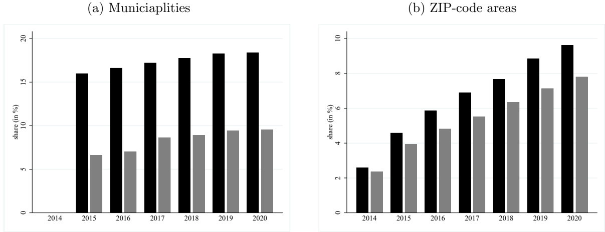
Figure 1: Stability of regional entities over time
